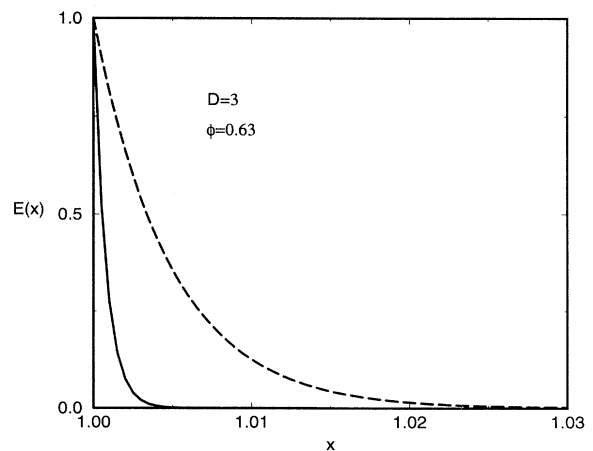
FIG. 5. Comparison of exclusion probability E(x) for hard spheres ( D = 3 ) of diameter \sigma vs dimensionless distance x = r/\sigma obtained from Eq. (42) (solid curve) and Eq. (5.22) (dashed curve) of Ref. [18] for \phi = 0.63 .
